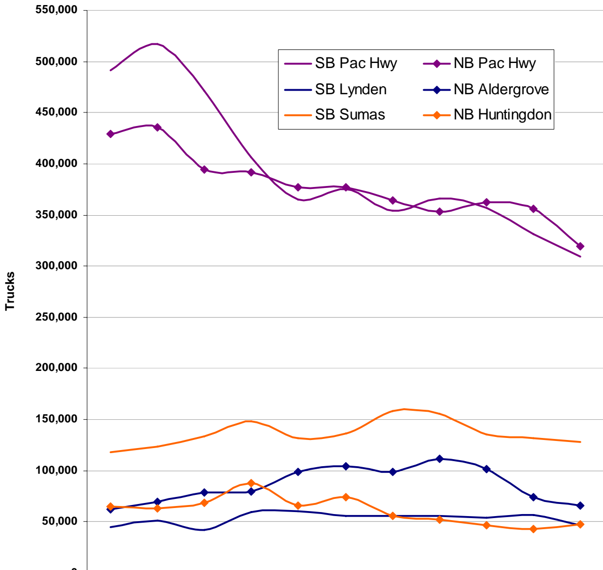
Chart 4. 1999–2009 Cascade Gateway Cross-Border Truck Counts, by Crossing, by Direction (SB = southbound, NB = northbound).
