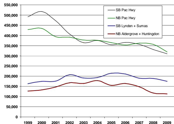
Chart 5: Volumes comparison – Pacific Highway Directional Volumes vs. Combined Lynden & Sumas SB Volumes and Aldergrove and Huntingdon NB Volumes. 1999 -2009
